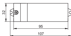
TRN 60M
