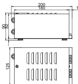
HQI 70, 150
